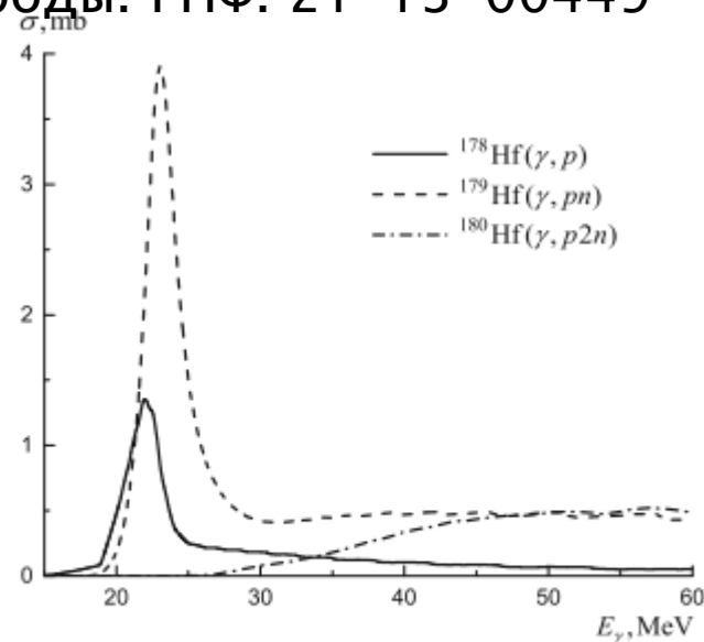
Fig. 1 Theoretical cross-sections of photonuclear reactions on \text{natHfO}_2 leading to ^{177}\text{Lu} formation calculated by TALYS and CMPR combination
