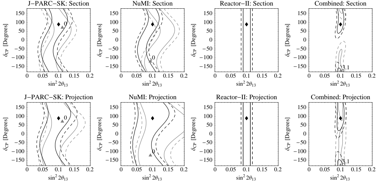
Figure 8: The 90% CL (solid curves) and 3\sigma (dashed curves) allowed regions (2 d.o.f.) in the \sin^2 2\theta_{13} - \delta_{\text{CP}} -plane for the true values \sin^2 2\theta_{13} = 0.1 and \delta_{\text{CP}} = 90^\circ for JPARC-SK, NuMI, Reactor-II. The right-most plots are calculated for the shown experiments in combination with the conventional beams. For the true values of the un-displayed oscillation parameters, we choose the current best-fit values and a normal mass hierarchy. The black curves refer to the allowed regions for the normal mass hierarchy, whereas the gray curves refer to the \text{sgn}(\Delta m_{31}^2) -degenerate solution (inverted hierarchy), where the projections of the minima onto the \sin^2 2\theta_{13} - \delta_{\text{CP}} -plane are shown as diamonds (normal hierarchy) and triangles (inverted hierarchy). For the latter, the \Delta\chi^2 -value with respect to the best-fit point is also given. The upper row shows the fit manifold section (with the un-displayed oscillation parameters fixed at their true values), and the lower row shows the projection onto the \sin^2 2\theta_{13} - \delta_{\text{CP}} -plane as the final result.
